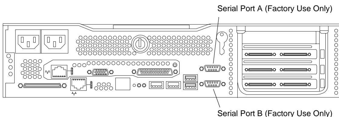
Figure 1. Rear Panel of hp 9000 rp3410/rp3440 Server
