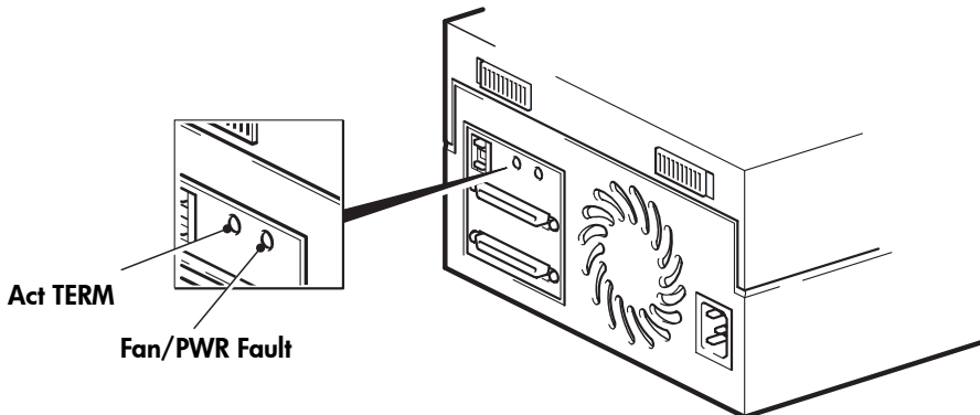
Figure 8c: indicators on rear of drive
