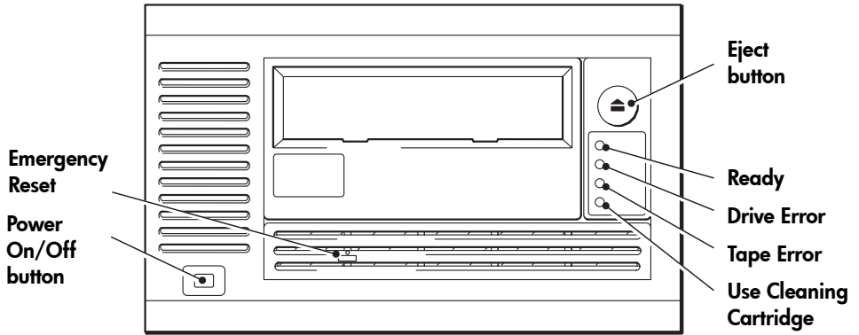
Figure 8a: Ultrium 230 tape drive controls and indicators
