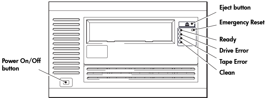
Figure 8b: Ultrium 960 and 460 tape drive controls and indicators
