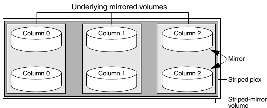
Figure 1-19 Striped-mirror volume laid out on six disks
