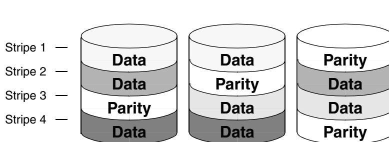
Figure 1-21 Parity locations in a RAID-5 mode
