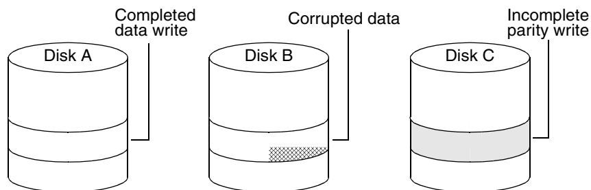
Figure 1-25 Incomplete write to a RAID-5 volume
