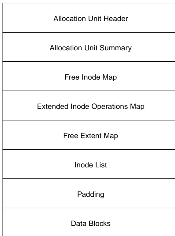
Figure 7. Allocation Unit Structure
