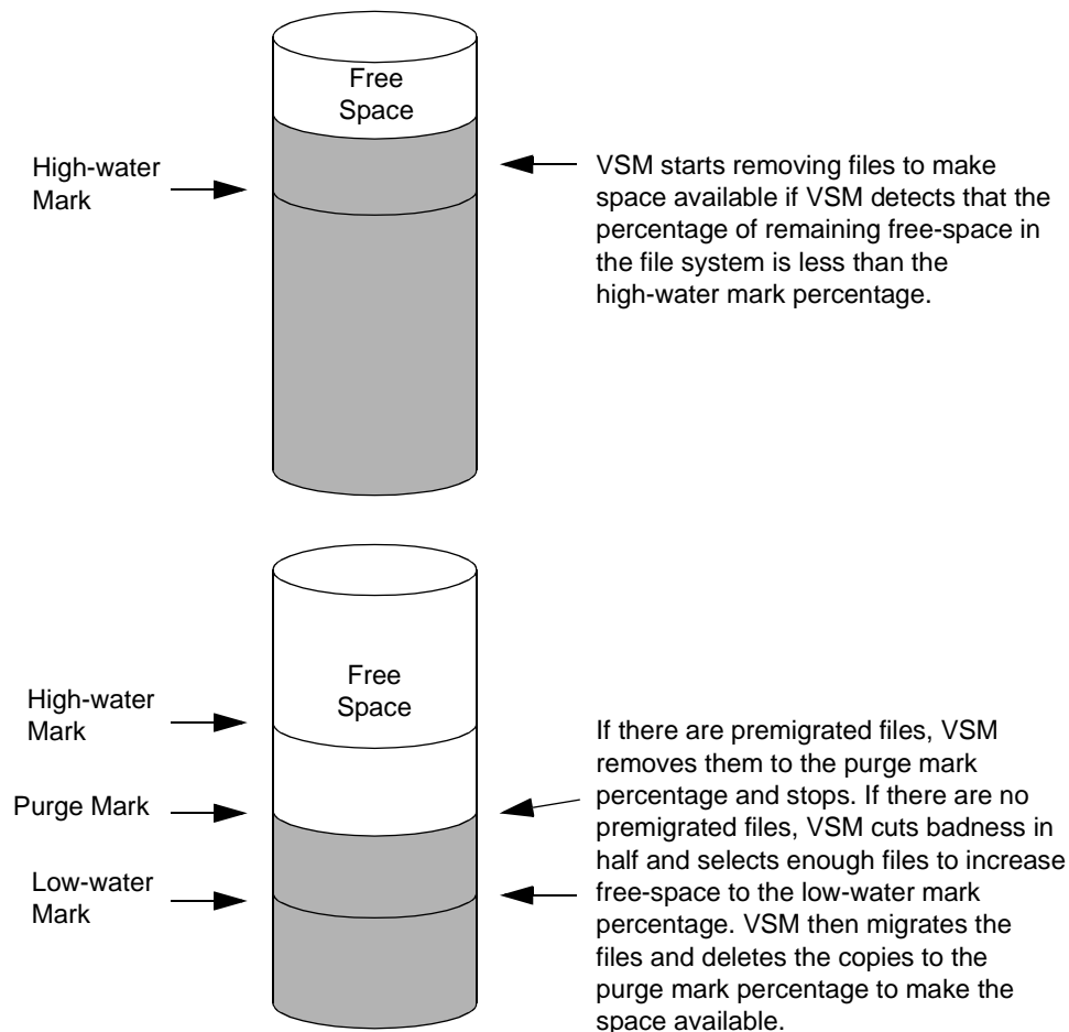
Figure 9. Migration Parameters
