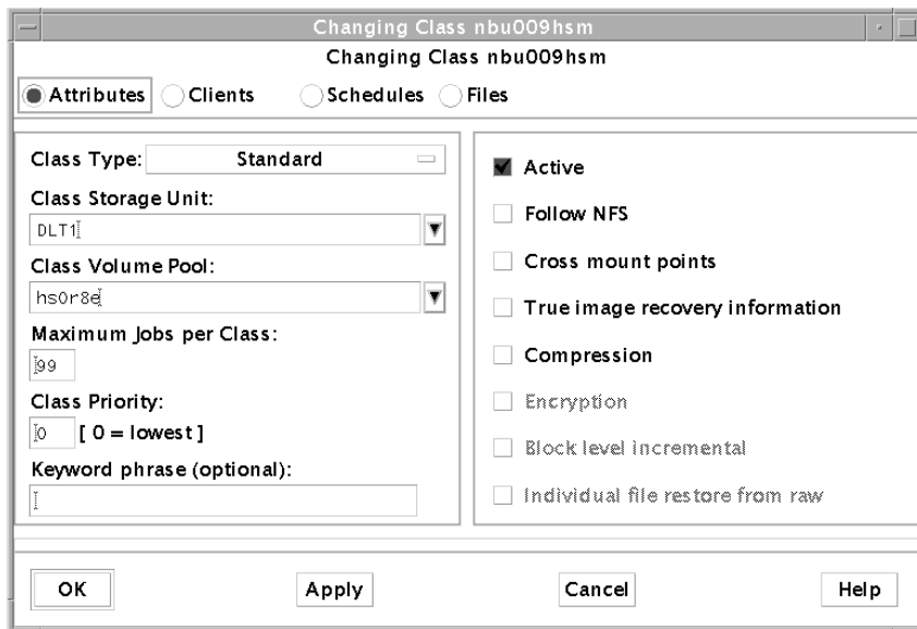
Figure 104. Class Attributes
