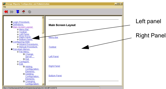
Figure 113. Help Dialog
