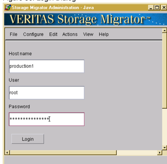
Figure 50. Login Dialog
