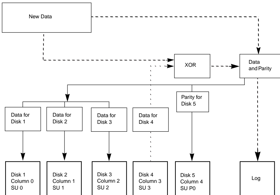
Figure 9 Reconstruct-Write
