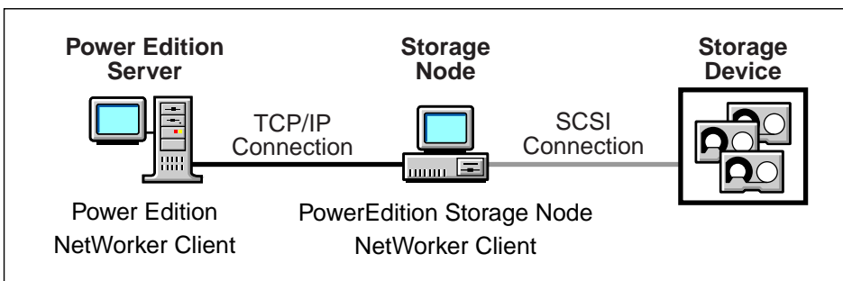
Figure 3. Power Edition Storage Node Backup and Recover
