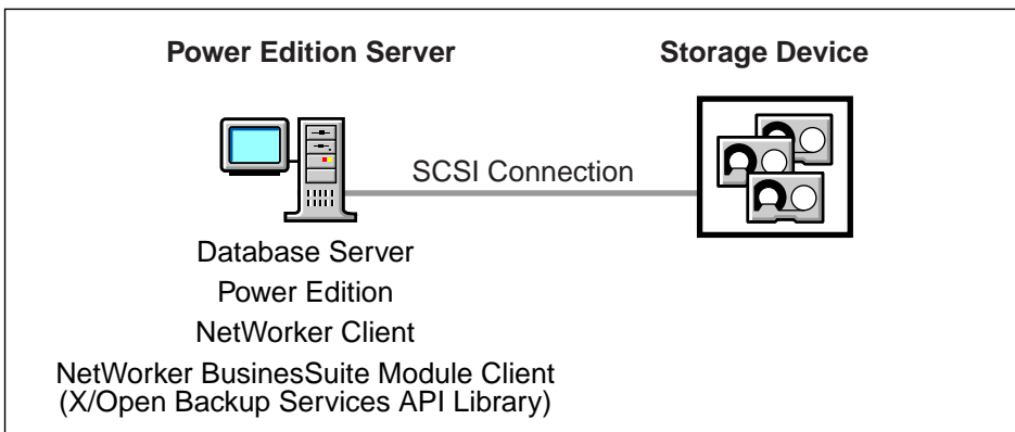
Figure 1. Local Backup and Recover
