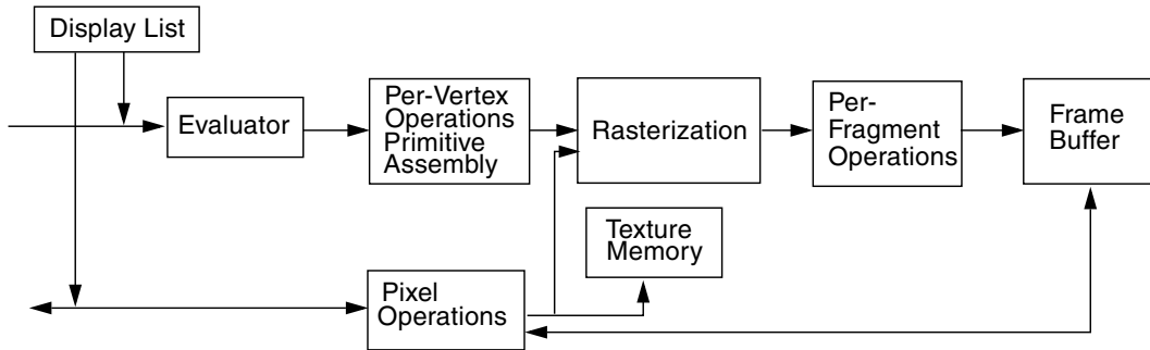
FIGURE 2-1 Basic Architecture
