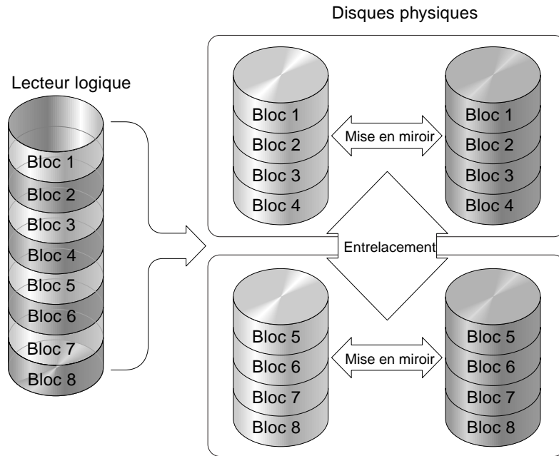
FIGURE A-9 Configuration RAID 1+0
