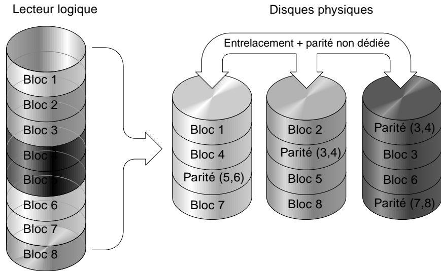
FIGURE A-11 Configuration RAID 5
