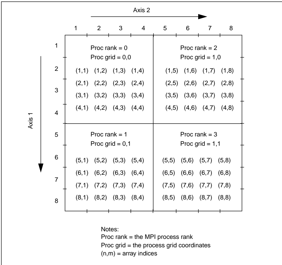
FIGURE 3-4 An 8x8 Sun S3L Array Distributed on a 2x2 Process Grid Using Pure Block Distribution: Column-Major Ordering of Processes
