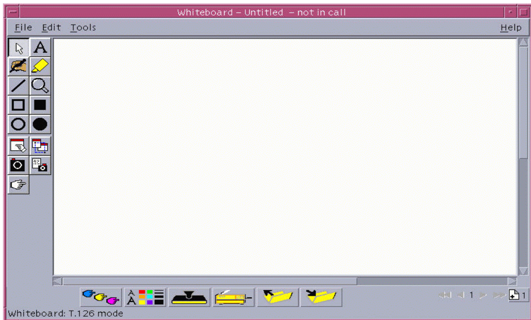
FIGUR 2-4 SunForum 3.2 Whiteboard
