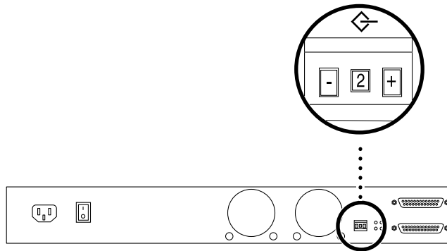
FIGURE 1-10 SCSI ID Switch
