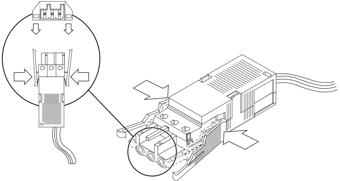
FIGURE 3-27 Disconnecting the DC Input Power Cable From the DC Connector
