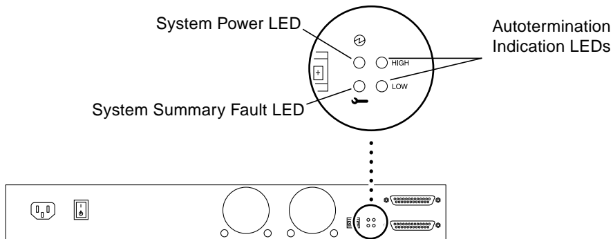
FIGURE 5-4 Back Panel LEDs
