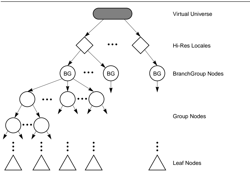
Figure 4-1 The Virtual Universe
