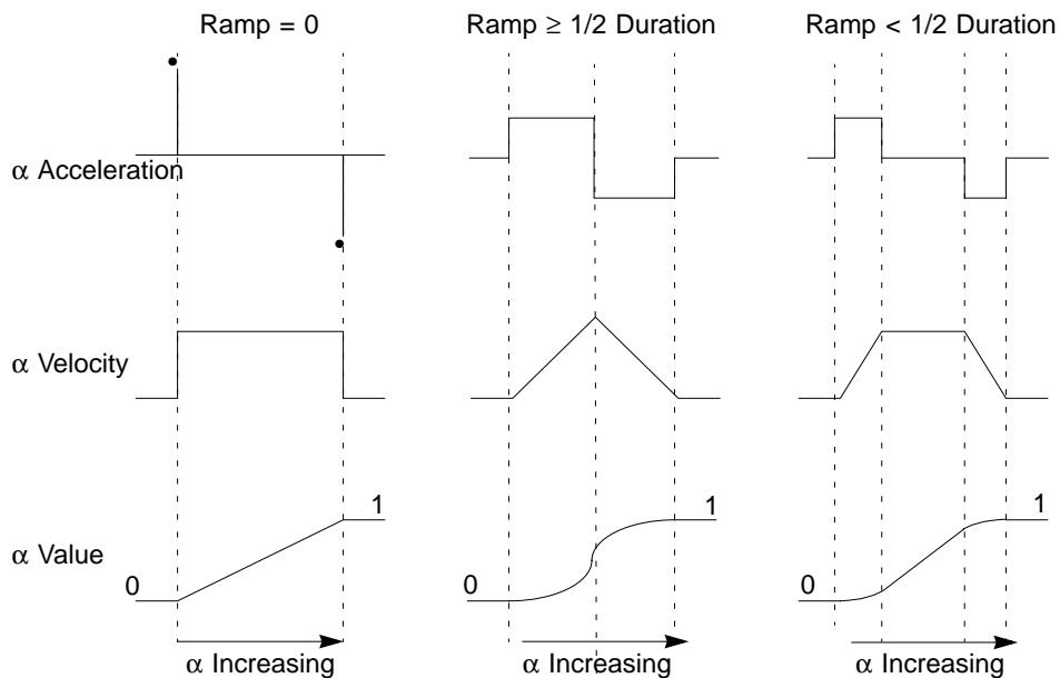
Figure 10-8 How an Alpha-Increasing Waveform Changes with Various Values of increasingAlphaRampDuration
