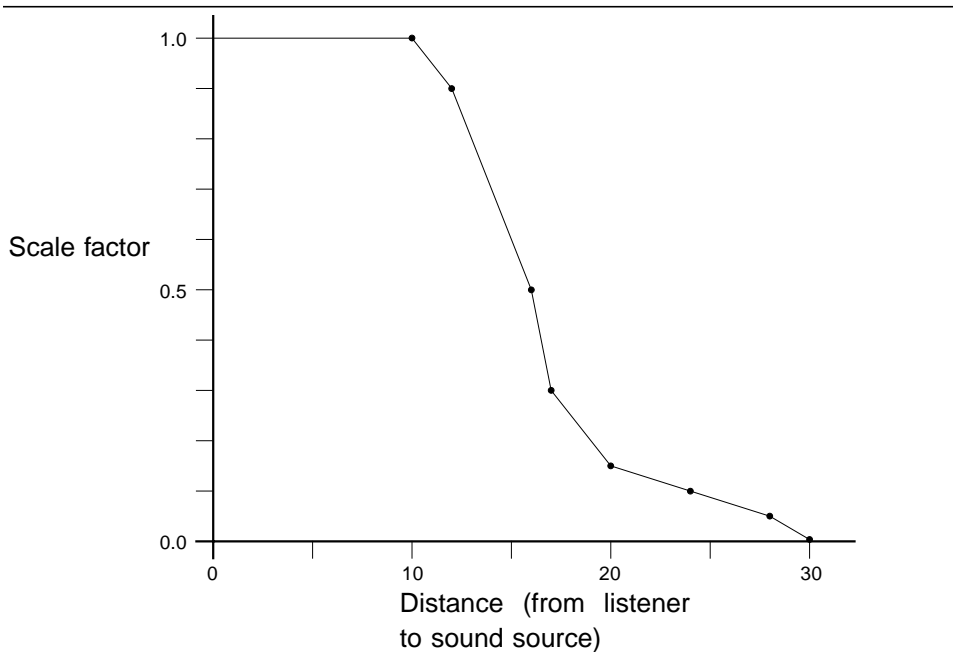
Figure 6-2 PointSound Distance Gain Attenuation
