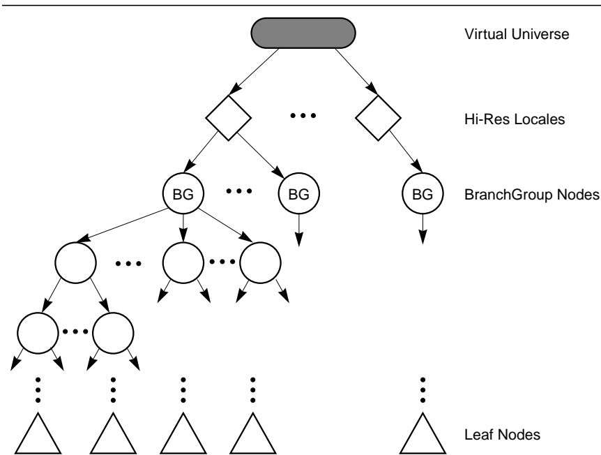
Figure 3-1 A Java 3D Scene Graph Is a DAG (Directed Acyclic Graph)
