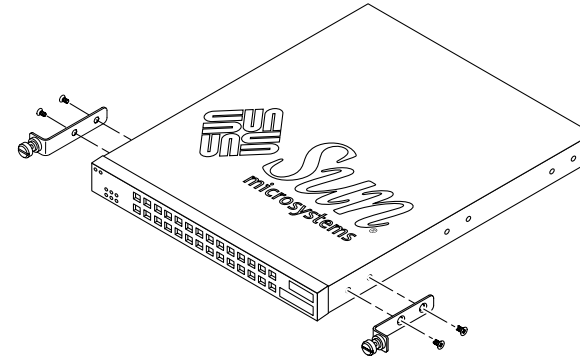
Figure 2 Installing the Thumbscrew Rack Brackets
