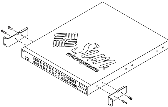
Figure 1 Removing the Rackmount Brackets
