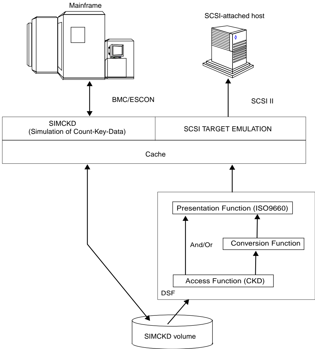
FIGURE 2-3 Mainframe DSF Capability Architecture
