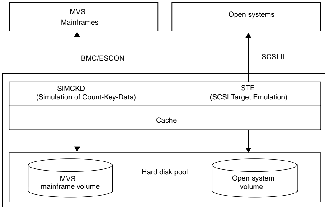
FIGURE 2-1 Product Architecture
