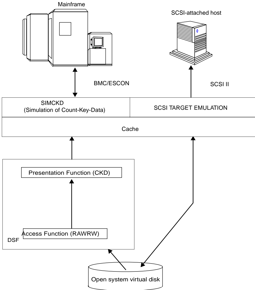
FIGURE 2-5 Backup/Restore DSF Capability Architecture
