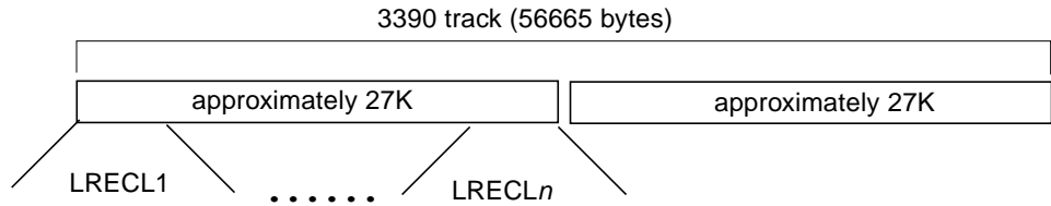
FIGURE 3-2 3390 Open Systems Capability Dataset Characteristics
