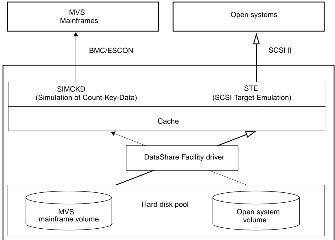
FIGURE 2-2 DataShare Facility Architecture
