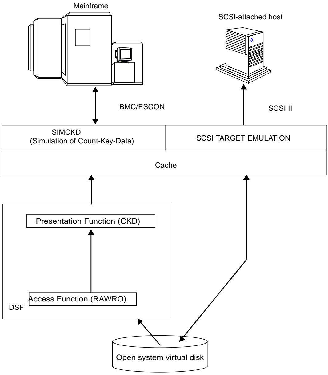
FIGURE 2-4 Open System DSF Capability Architecture
