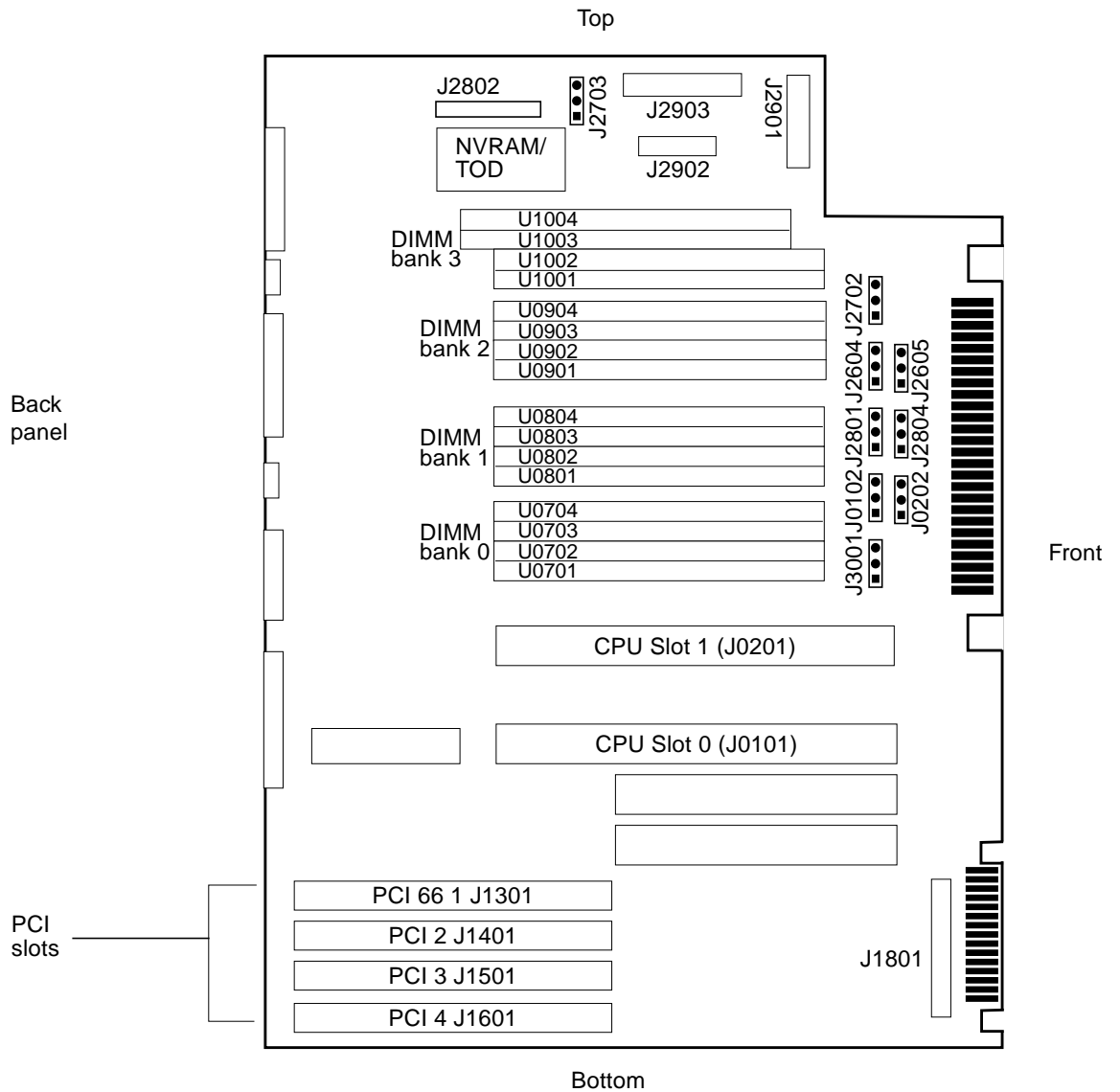
FIGURE 4-4 PCI Card Slot Locations on the Motherboard
