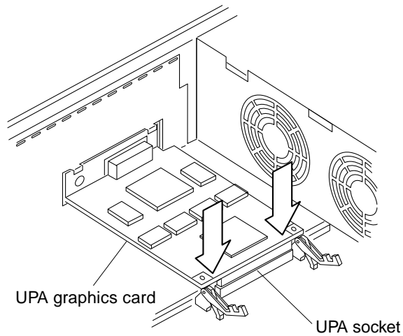
FIGURE 4 Seating the UPA Graphics Card into the Socket
